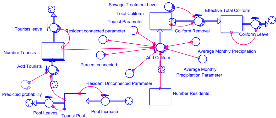
Figure 5.2. Ecologic Submodel
